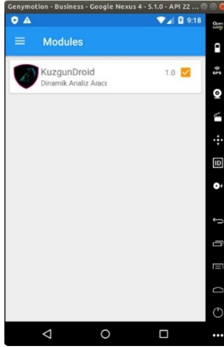
Figure 8. KuzgunDroid module
