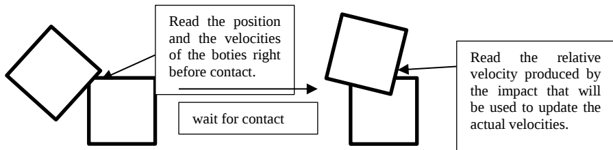
Figure 3: A Detailed Illustration of the Procedure for Generating Training Data Utilizing the Physics Engine
