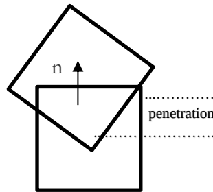
Figure 2. Detailed Visualization of the Narrow Phase Collision Detection Mechanism Focusing on Box-against-Box Interactions Source: Author's own conception
