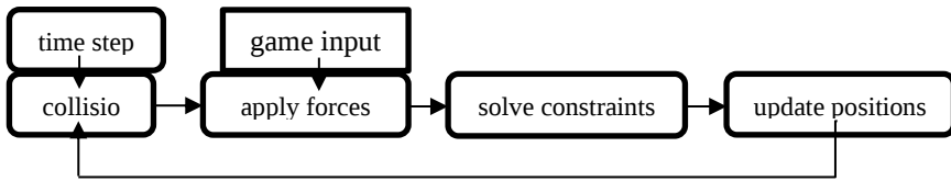
Figure 1. Illustration of the Operational Loop in the Box2D-Lite Physics Engine Source: Author's own conception
