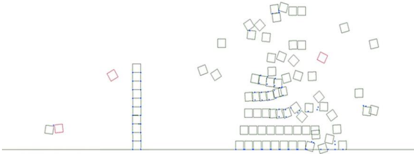
Figure 4: The Illustrated Scenarios Used for Training Data Generation; Scenario 1 Demonstrating a Single Object Interaction, Scenario 2 Demonstrating Interaction of a Single Object with a Stack of Ten Additional Objects, and Scenario 3 Highlighting a Complex Interaction Involving a Pyramid Comprised of Sixty-Six Objects
