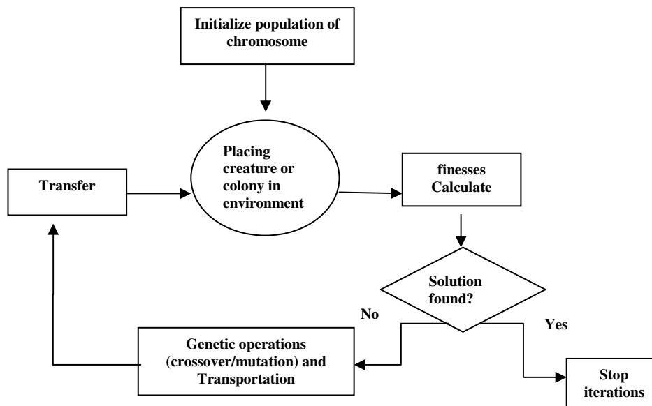
Figure 12. Genetic Algorithm flowchart
