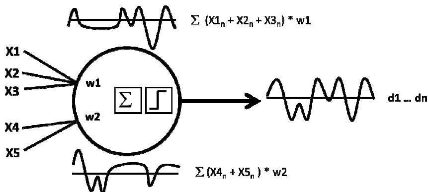
Figure 2. New neuronal model, based on matching a wave-like representation of the output.
