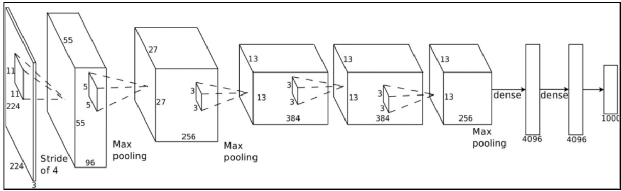
Figure 1. CNN architecture (adopted from Krizhevsky et al. '12)
