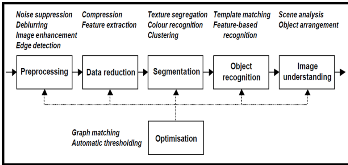
Figure 1. Methodology used in the research by (Egmont-Petersen et al., 2002)
