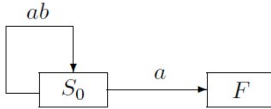
Figure 3. Representation of the grammar G_1 in the labelled graph G_0^1
