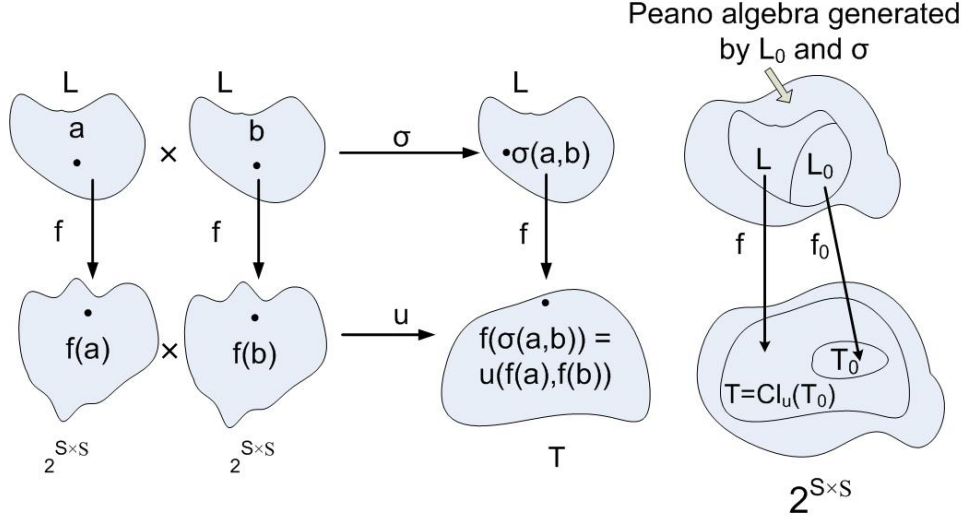
Figure 1. The graphical representation of the morphism f: (L, \sigma_L) \rightarrow (2^{S \times S}, \sigma_T) (Țăndăreanu, 2000)
