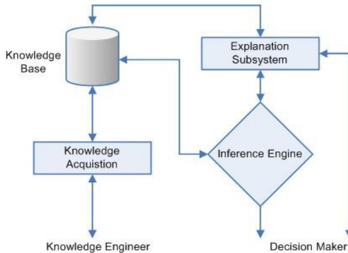
Figure 1. Rule Based System Cycle
