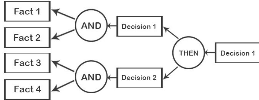
Figure 4. Backward chaining cycle
