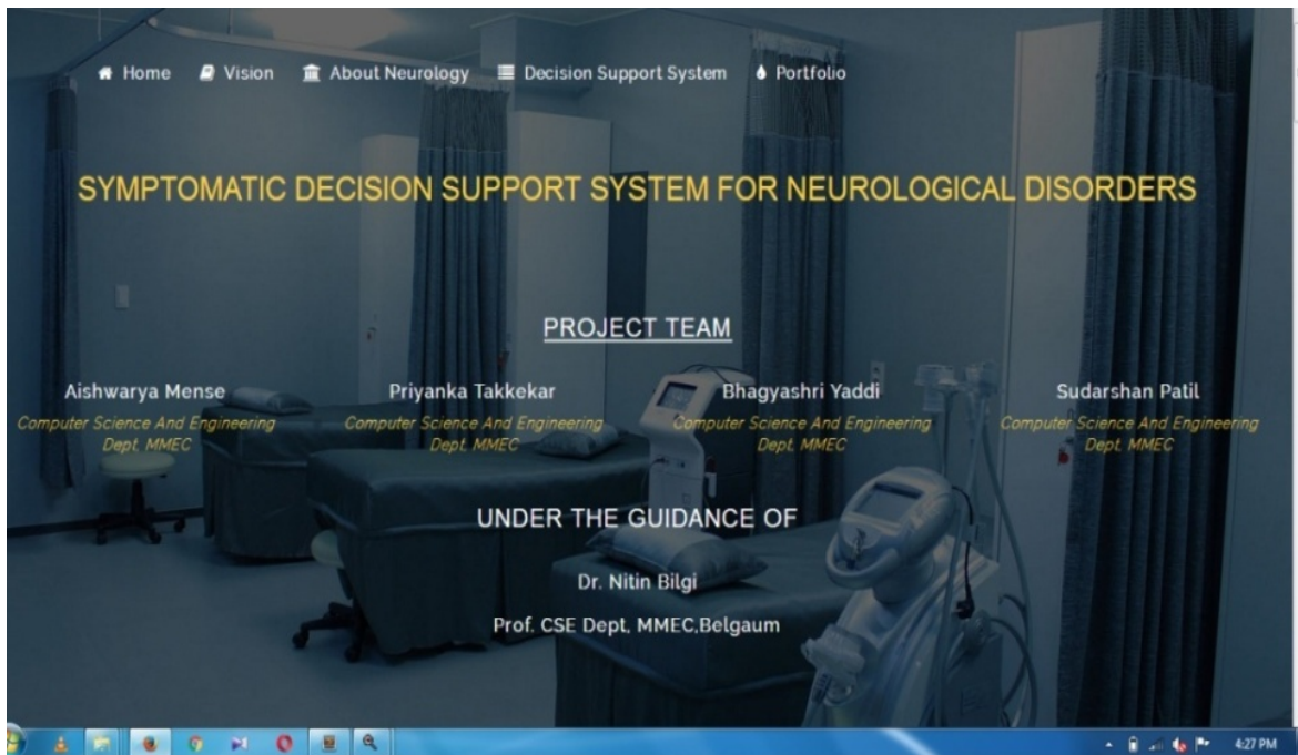
Figure 6. Home page
