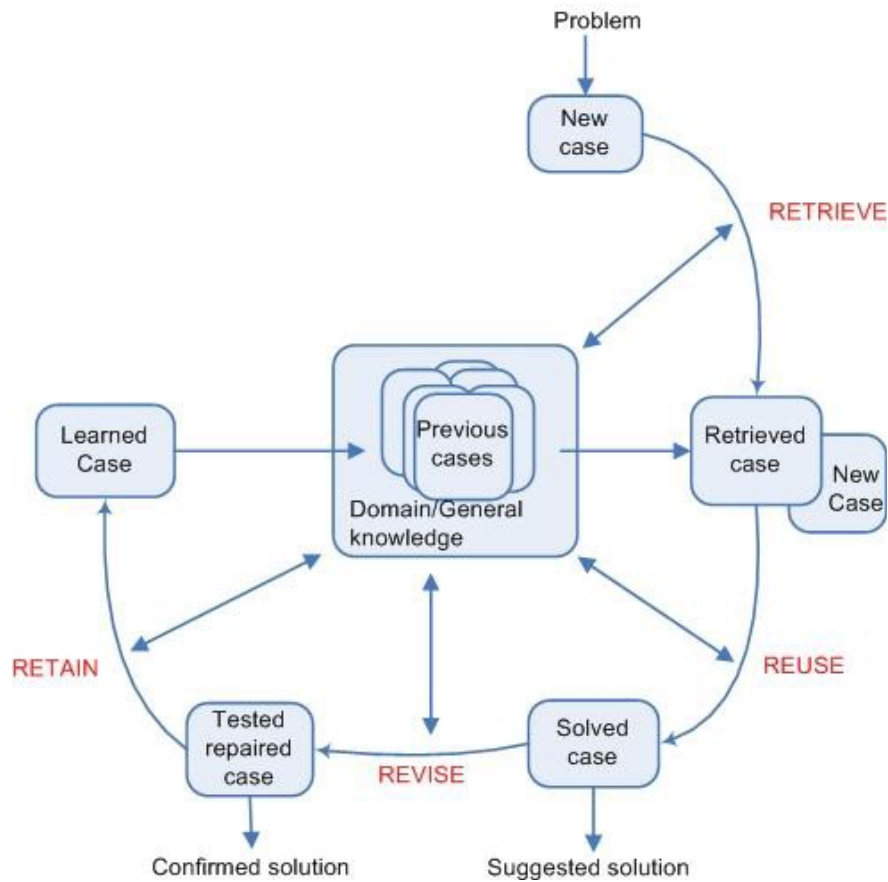
Figure 5. Case-Based Reasoning Cycle
