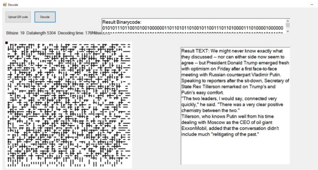
Figure 14. QR code decoded and result shown.
