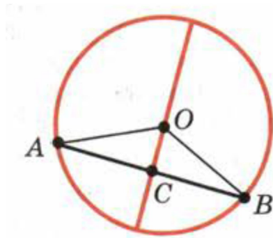
Figure 2. A circle, a chord, and a diameter
