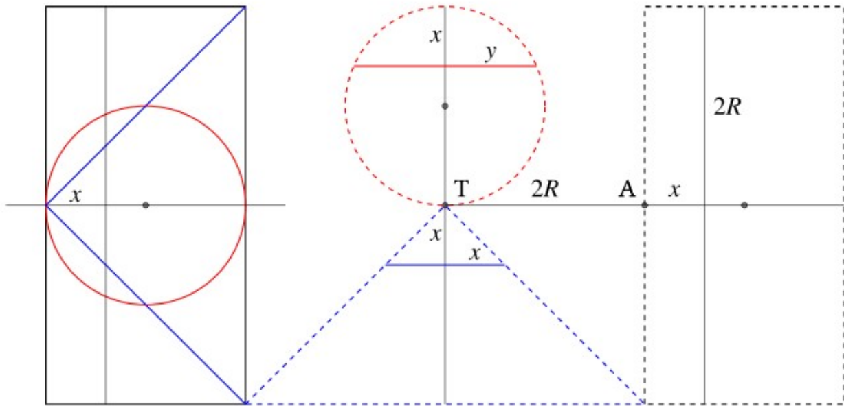
Figure 6. Archimedes: determining the volume of the ball inscribed to the cylinder
