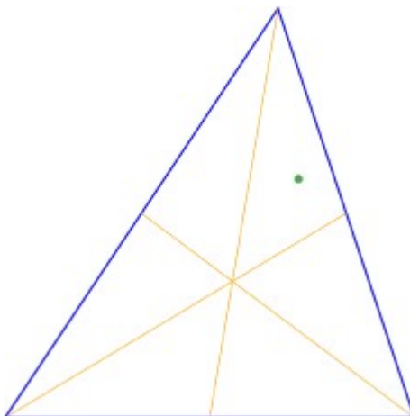
Figure 3. A triangle with medians and “one” point
