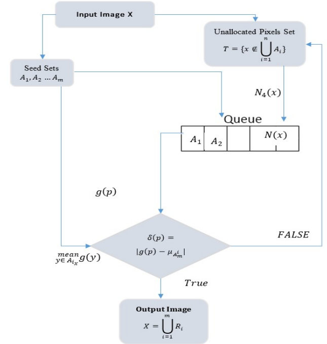
Figure 2. Predicate Mechanism for Non-Parametric SRG
