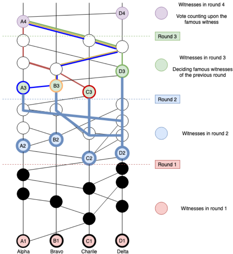
Figure 1 - Hashgraph and the consensus algorithm
