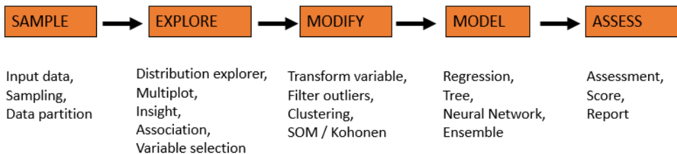
Figure 2. SEMMA methodology
