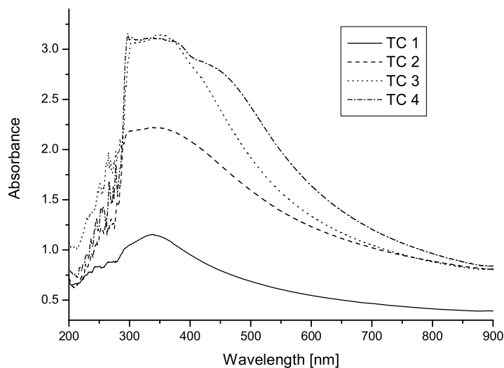
Figure 3: Absorption spectra of \text{TiO}_2/\text{CdS} composites samples with a different mass proportion
