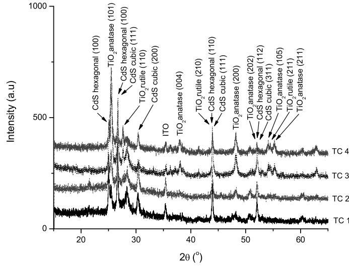
Figure 1: X-ray diffraction pattern for \text{TiO}_2/\text{CdS} composites samples
