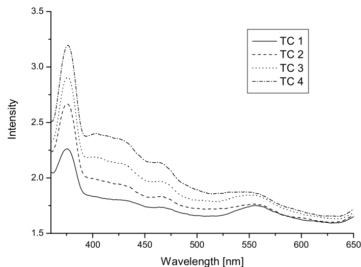
Figure 4: Spectrofluorimetric spectra of \text{TiO}_2/\text{CdS} composites samples with a different mass proportion
