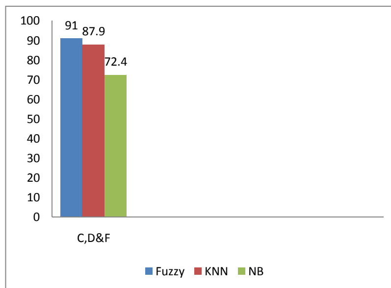
Figure 2 Bar chart represents the percentage of the correct diagnosis using fuzzy diagnosis, K- nearest neighbor and Naïve Bayes classifiers.
