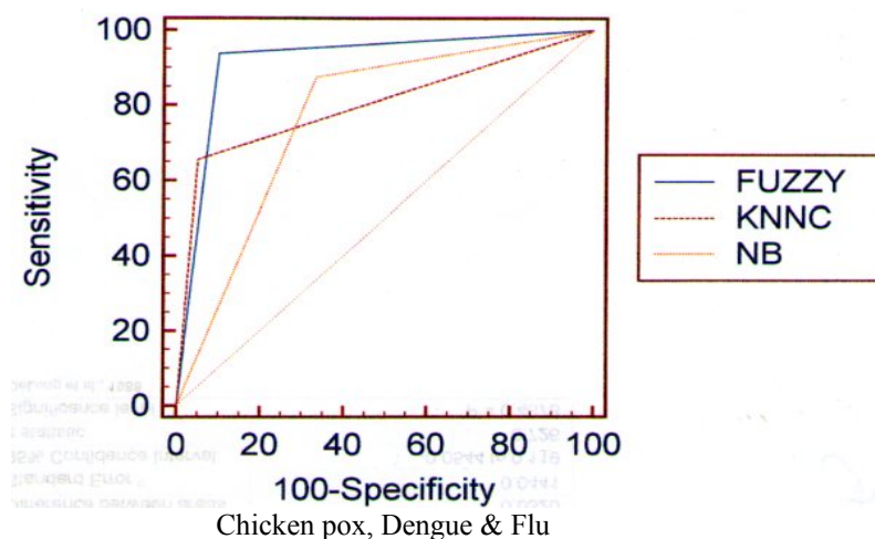
Figure 1. The comparison of the Area Under the ROC Curve (AUC) for fuzzy Diagnosis, KNN and NB
