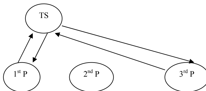
Figure 1. Cristian's Algorithm
