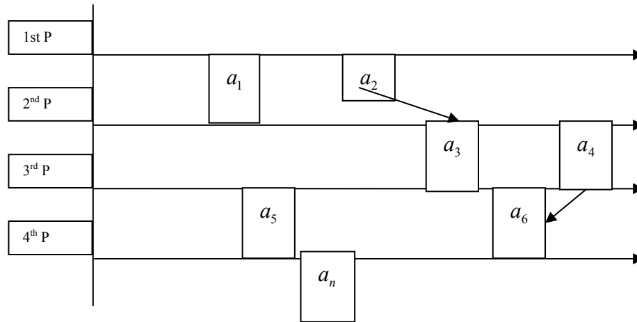
Figure 2. Lamport's algorithm
