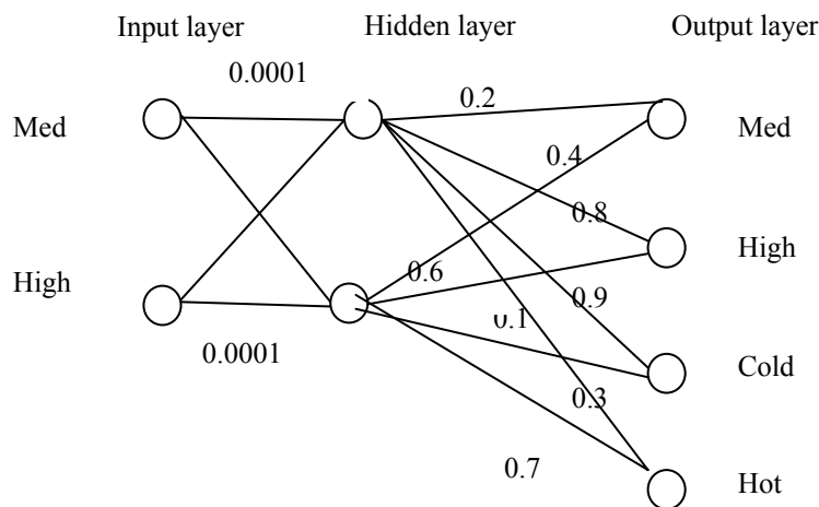
Figure 3. Neural network representation for HMM given in Figure 2.
