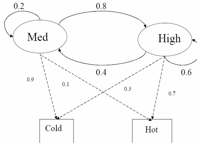
Figure 1. HMM to describe a relation between the states Med. and High with the observations (invisible states) cold and hot.
