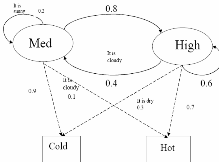
Figure 2. HMM with weights and necessary conditions on top of edges
