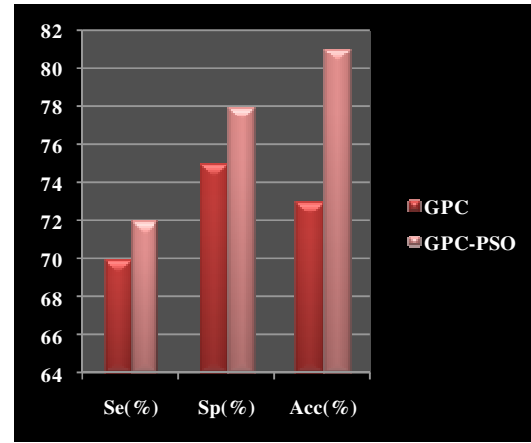
Figure 8(b). Comparing Se, Sp and Acc of GPC and GPC-PSO
