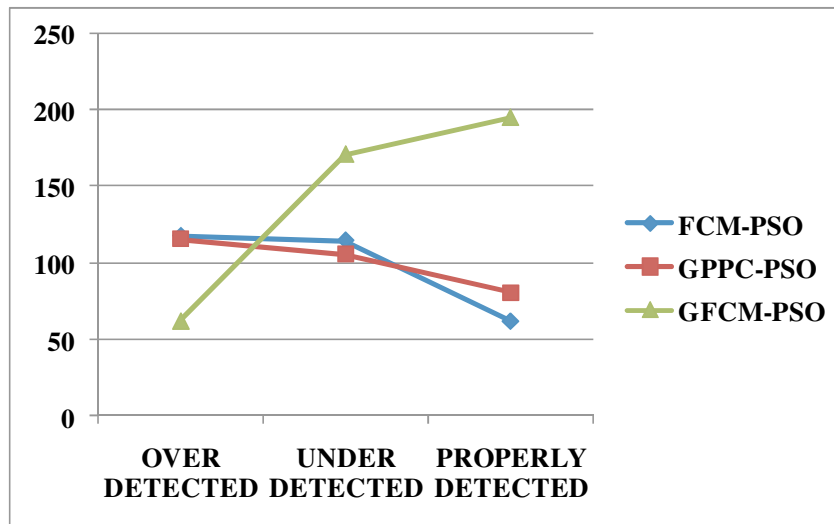
Figure 9. Performance analysis of FCM-PSO, GPC-PSO and GFCM-PSO
