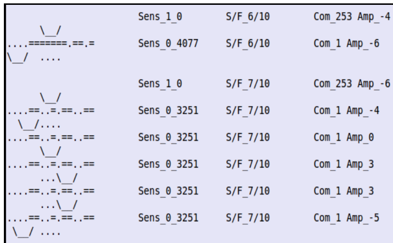
Figure 10.a. Simulation's display: The characters “\_/” represents the front part of the car that should pass through the string “....=..=..=..=” representing the range of obstacles
