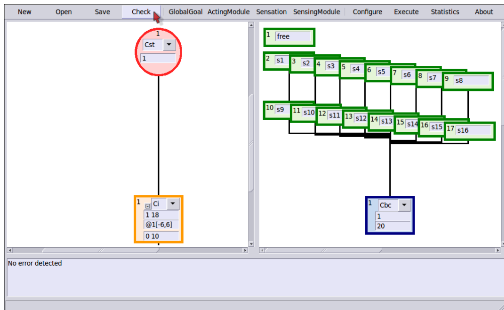
Figure 6. Adding a Global Goal with its required type
