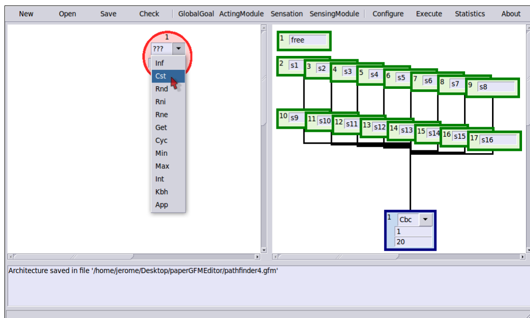
Figure 7. Adding an Acting Module, its configuration values and its input connections
