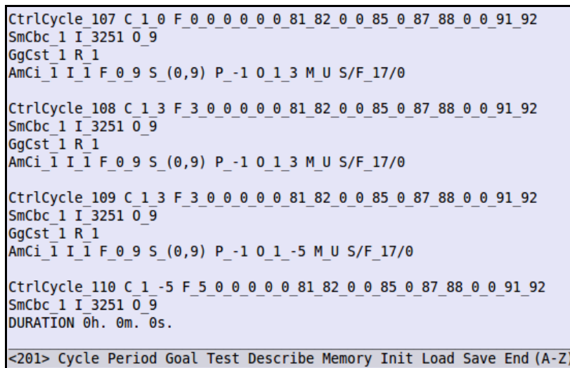
Figure 10.b. The control loop's information displayed by the controller
