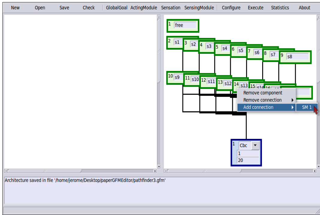
Figure 4. Adding a Sensing Module and selecting its type
