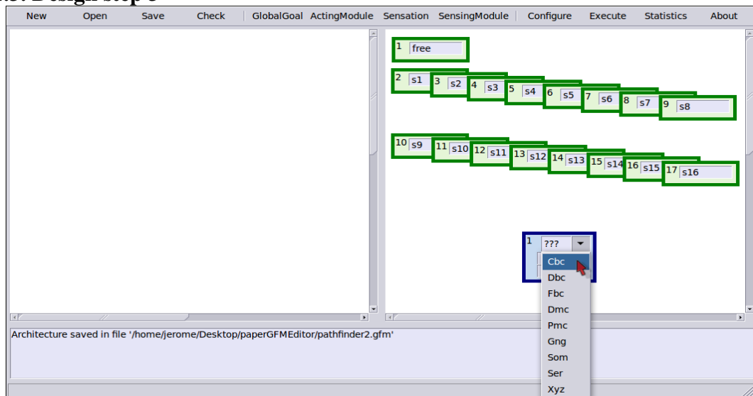
Figure 5. Adding connections from Sensations 2-17 to the Sensing Module 1
