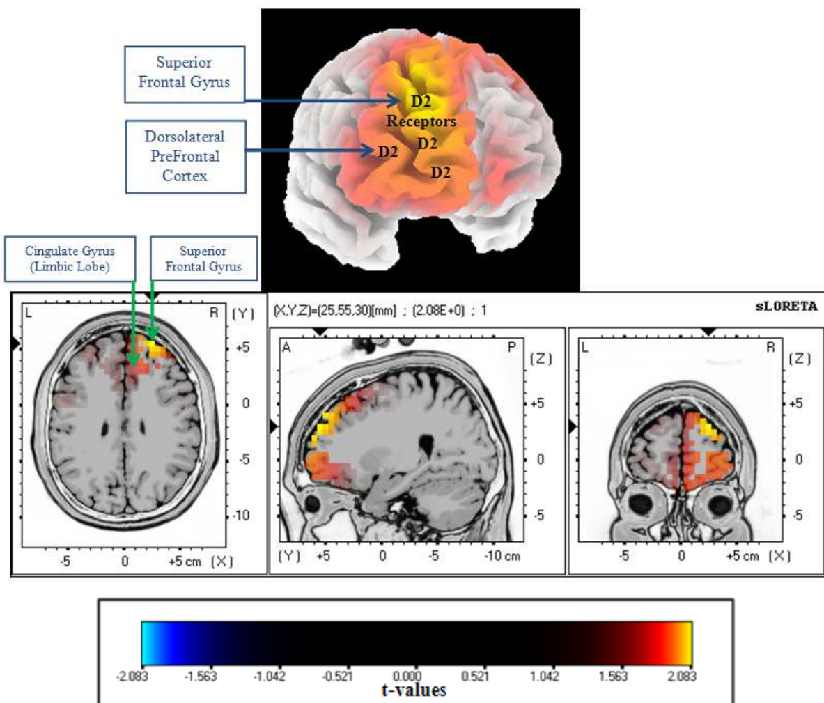
Figure 2. Resting State neuroimaging findings illustrating the action of atypical antipsychotics on post-synaptic dopamine D2-receptors following whole brain voxel-by-voxel unpaired t-tests that are based on statistical non-parametric map (SnPM) of sLORETA images in 100 Schizophrenia patients. The Yellow/Orange shades indicate increased neuronal activity in the delta frequency band in the right Superior Frontal Gyrus (Brodmann Area=10; MNI: X=25, Y=55, Z=30) along the dopamine mesolimbic pathway. Structural anatomy is shown in grey scale
