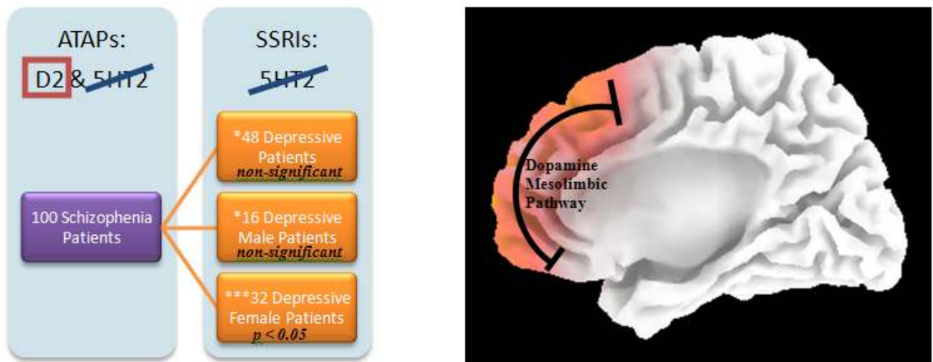
Figure 3. Resulting comparisons isolating the Dopamine D2 Mesolimbic Pathway using statistical non-Parametric Mapping (SnPM) indicating statically significant ( p < 0.05 ), via unpaired t-tests, results of 100 Schizophrenia patients medicated with Atypical Antipsychotics (ATAPs) compared with 32 Depressive patients medicated with Selective Serotonin Reuptake Inhibitors (SSRIs). *Indicates the non-statistically significant findings. ***Indicates the group SnPM pathway with statistically significant p < 0.05 findings.
