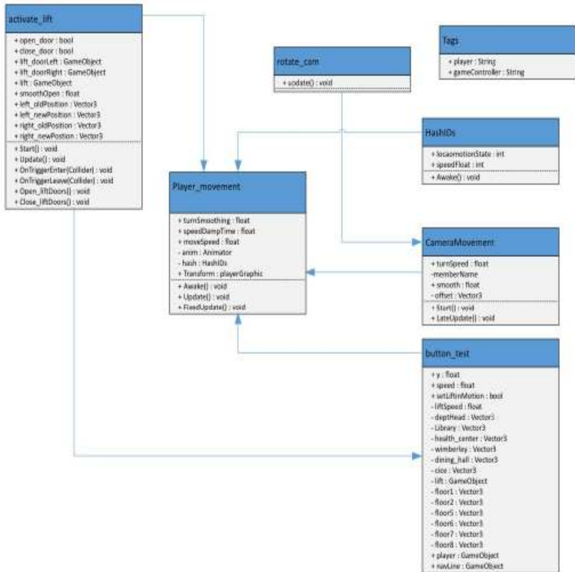
Figure 2. The class diagram for the Player and Camera movements
