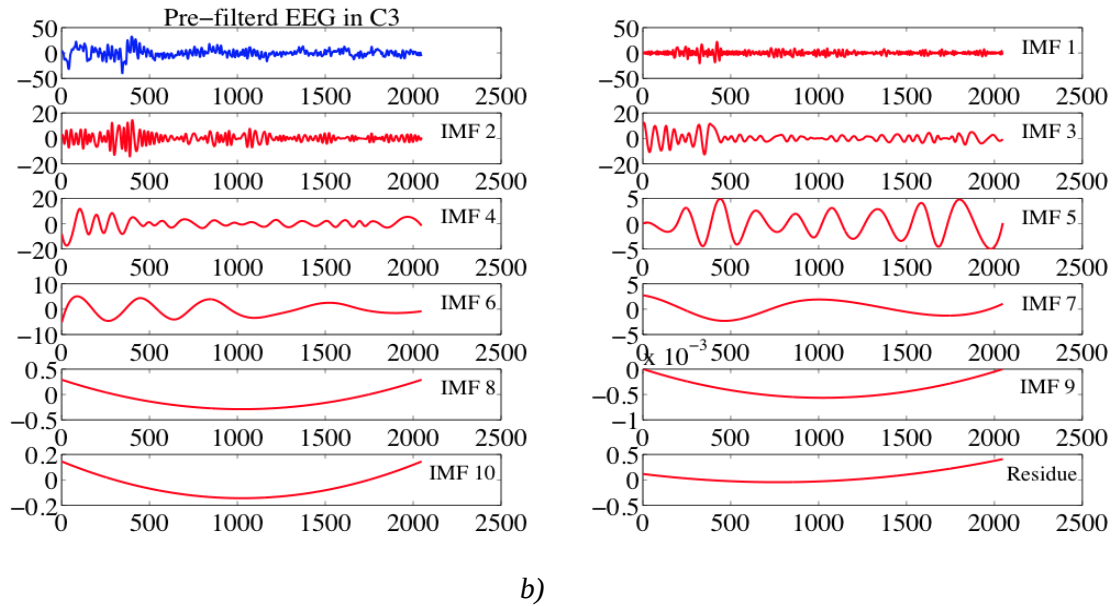
Figure 4. The EMD decomposition results for subject 2 when he imagines left hand movement. From top-left to down-right: the raw signal, the ten IMFs and the residue in channel C4 (a) and in C3 (b)
