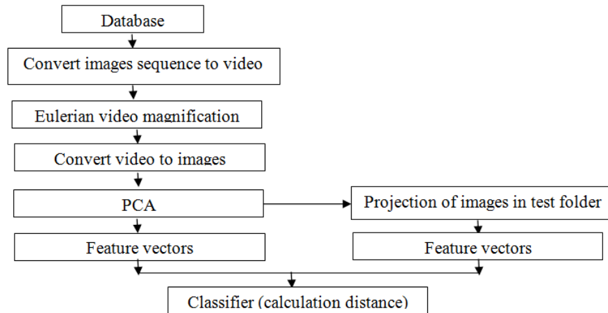
Figure 1. Overall structure of micro expression recognition
