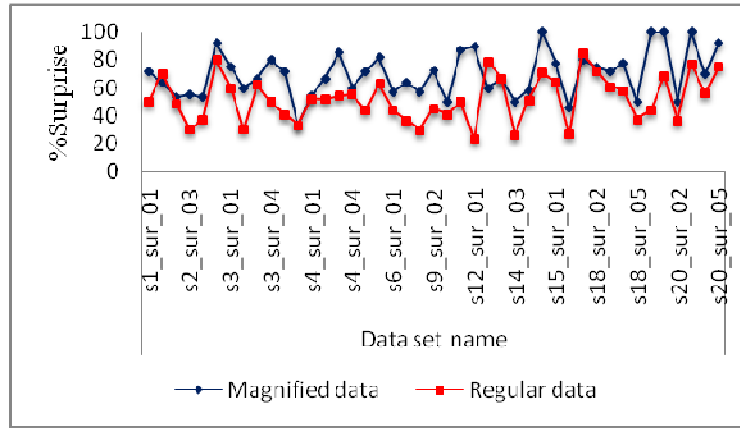
Figure 3. The chart of emotional/unemotional detection on the face in negative, positive and surprise states (Regular and magnified data)
