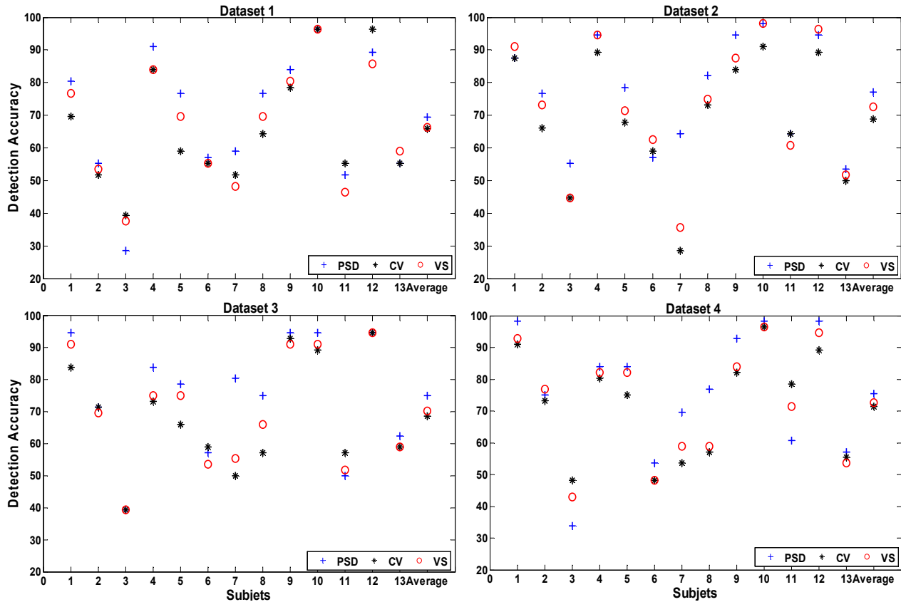
Figure 5. SSVEP detection accuracies by using PSD, CV and VS features
