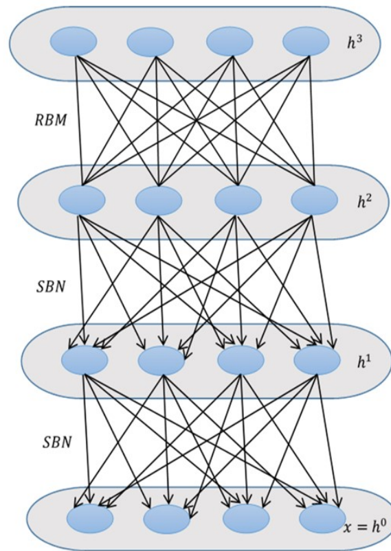
Figure 4. A DBN with three hidden layers, top layer forms an RBM and others form SBN
