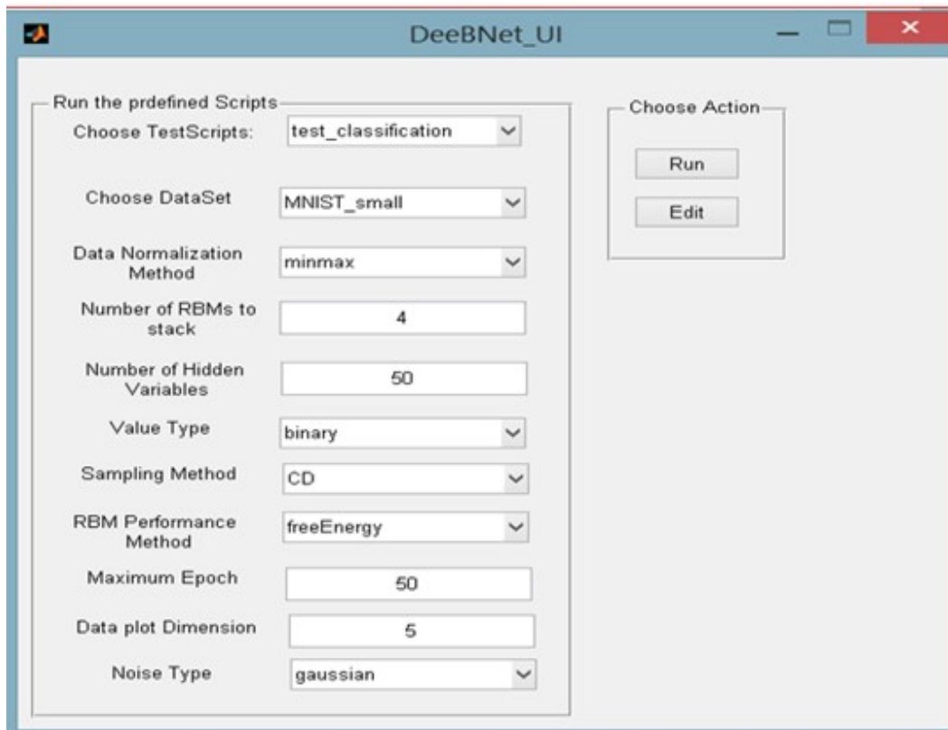
Figure 6. GUI Developed for working with DeeBNet Toolbox
