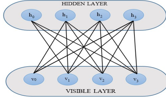
Figure 2. Structure of an RBM with 4 visible and 4 hidden units
