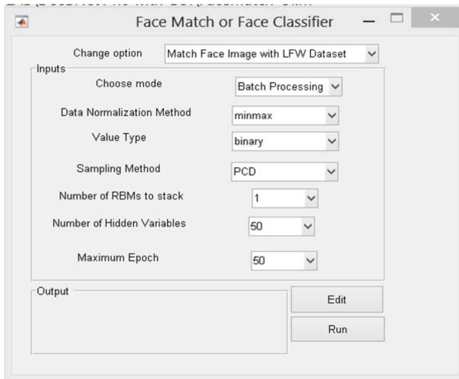
Figure 11 Front-End of Face Classifier
