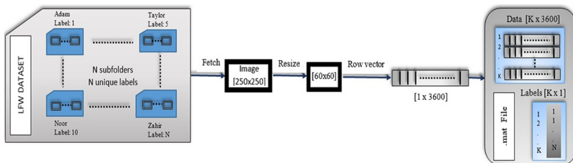
Figure 8. A pictorial representation of the conversion of LFW Dataset into Data Matrix with multiple labels
