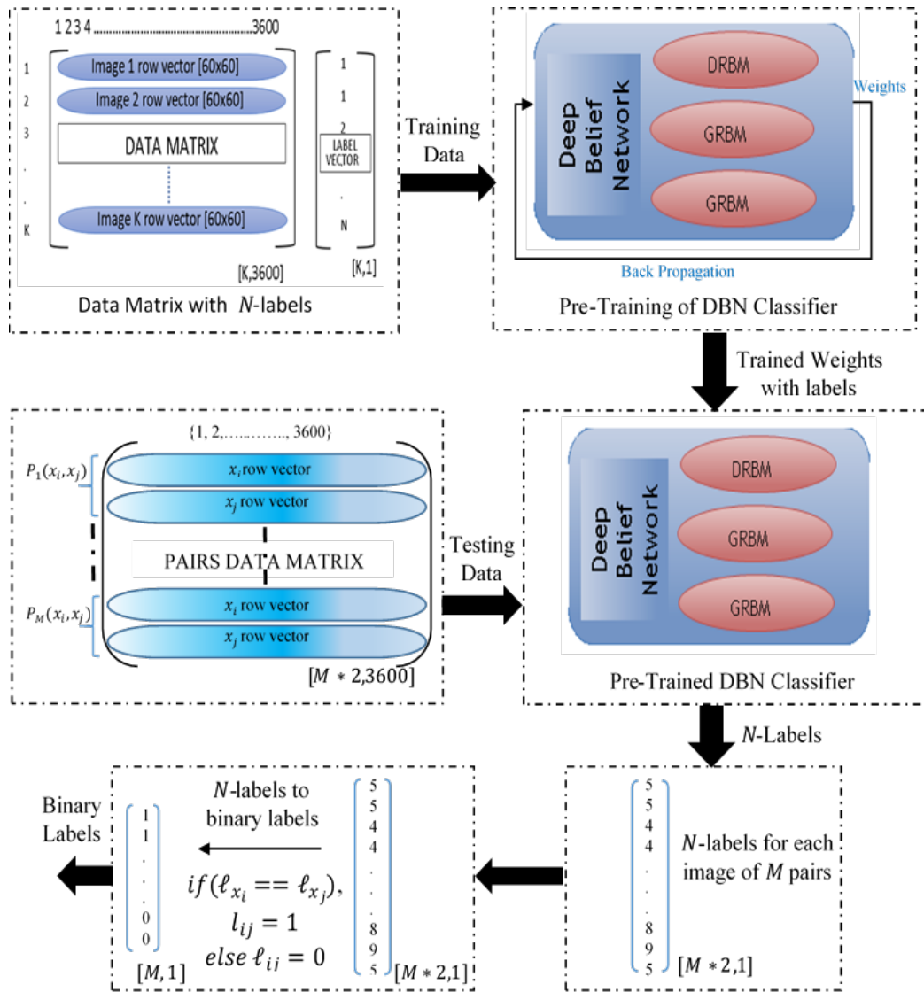
Figure 14. DBN Supervised Training and Transforming N -Way classification problem to 1-Way
