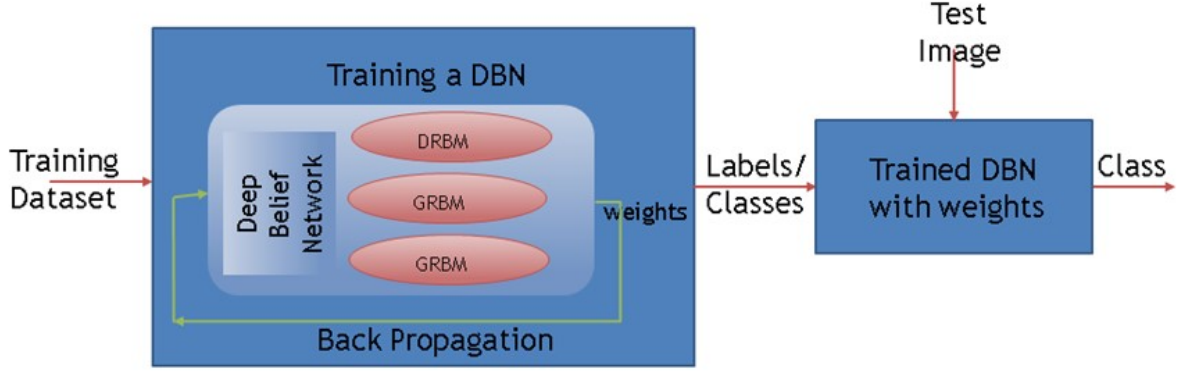
Figure 12. Workflow of DBN Classifier
