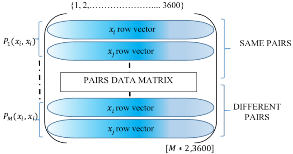
Figure 13. Training DBN using pair images
