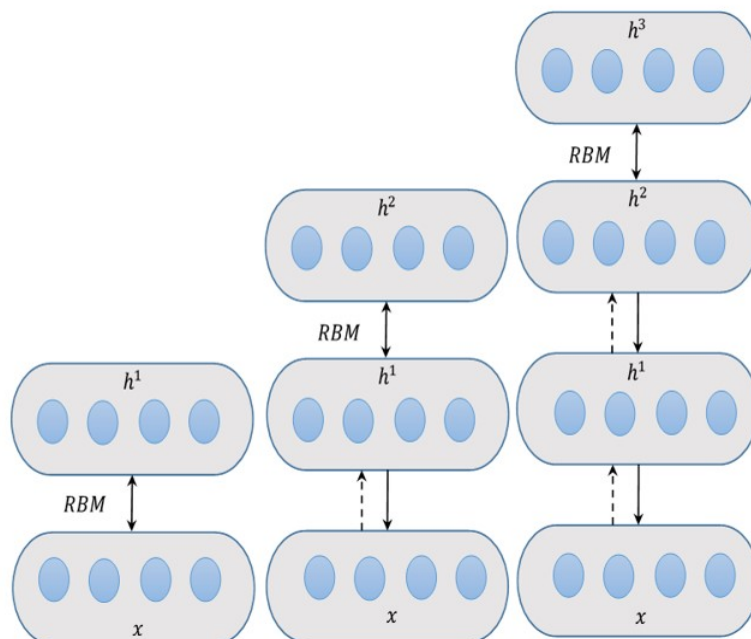
Figure 5. DBN as a stack of RBMs with layer-wise structure. The top layer always forms an RBM while the rest of the layers are SBNs. The generative path is shown with bold arcs and the recognition path is shown with dashed arcs.
