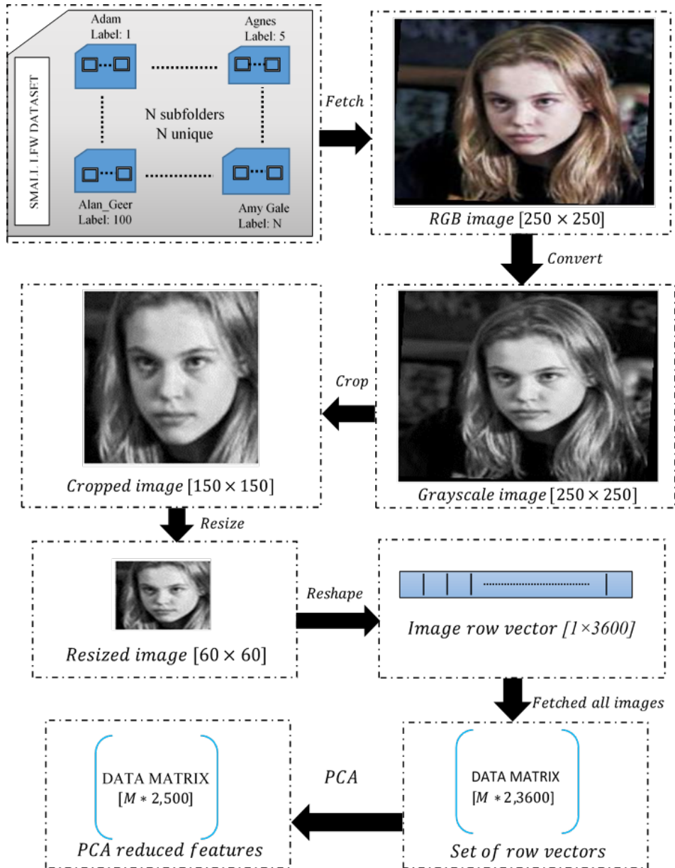
Figure 10. Flow of feature extraction with PCA
