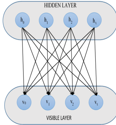
Figure 3. Structure of an SBN with 4 visible and 4 hidden units
