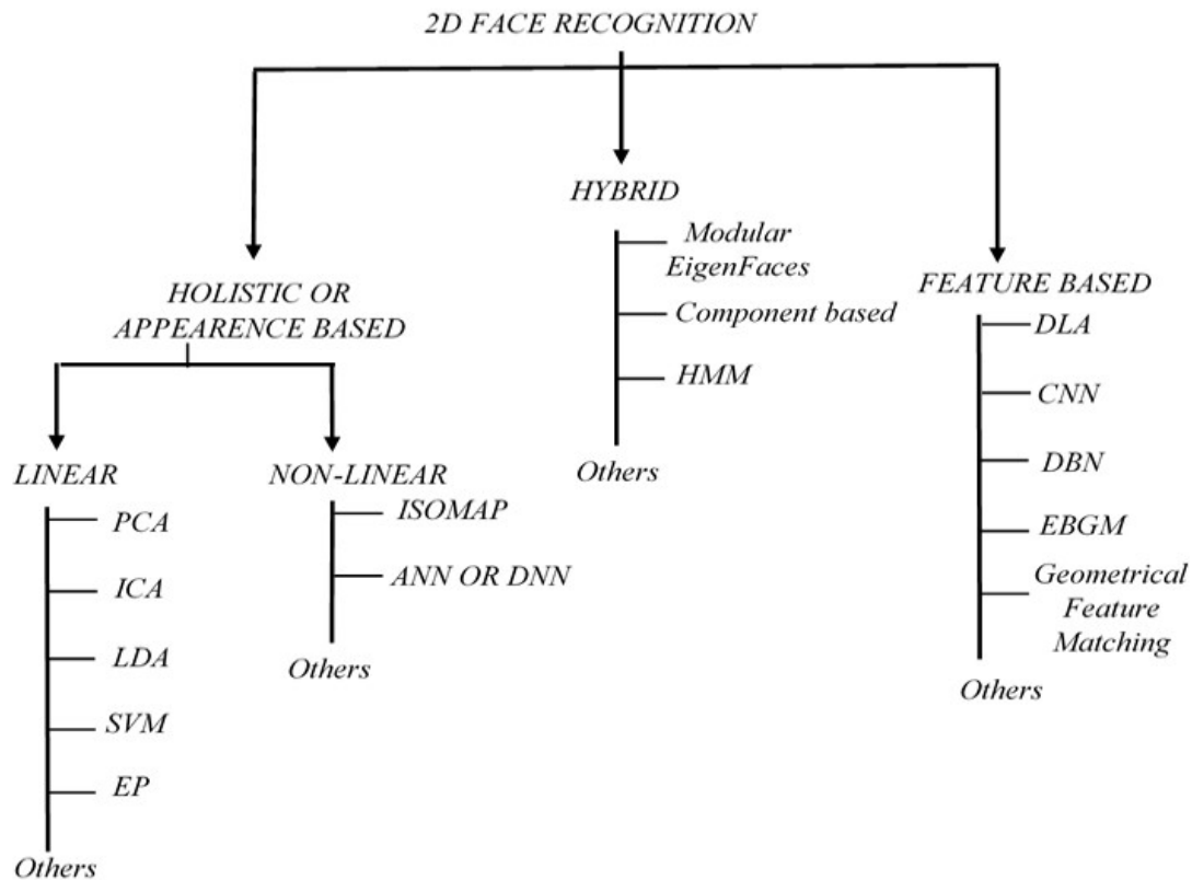
Figure 1. Overview of 2D image Recognition and classification approaches
