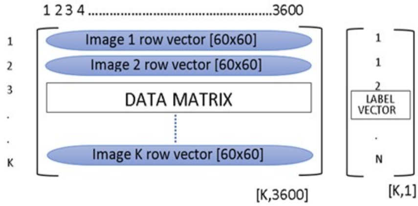
Figure 9. Design of the Data Matrix and Label Vector
