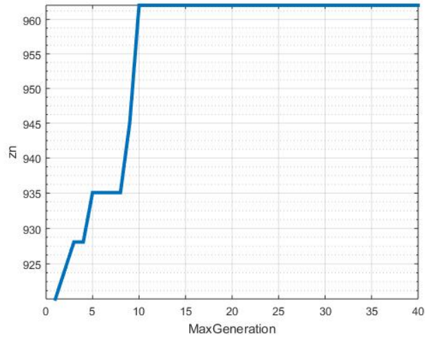
Figure 9. The relationship of the objective function with iterations; (case: \lambda = 20.451 , \mu = 0.04247 )
