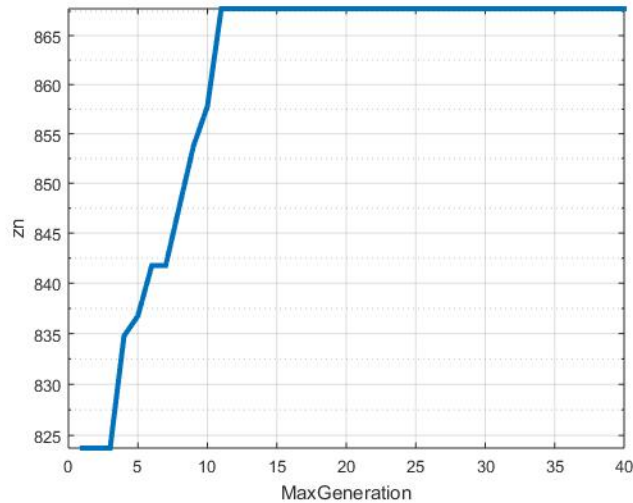
Figure 7. The relationship of the objective function with iterations; (case: \lambda = 19.938 , \mu = 0.0459 )
