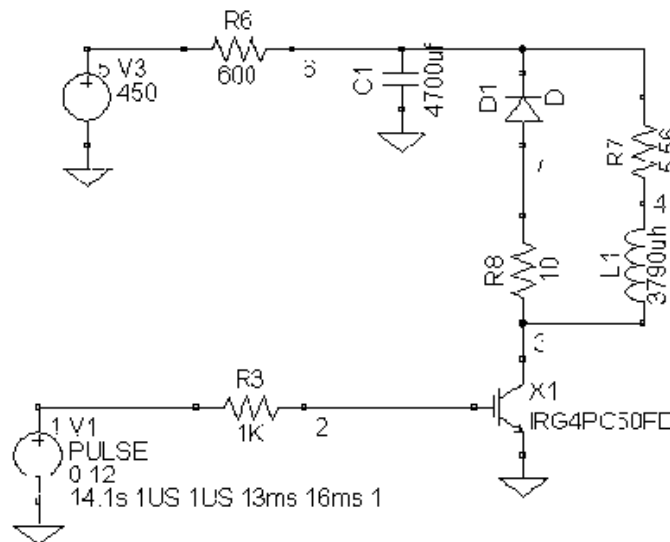
Figure 5. The solenoid controlling circuit design
