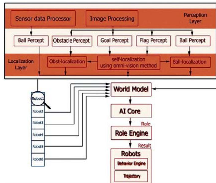
Figure 7. World model construction and artificial intelligent structure.
