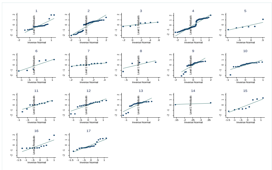
Figure 4: Q-Q plots line-up for level-1 residuals
