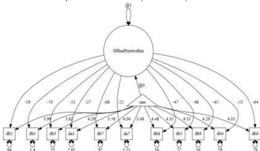
Figure 1: Path diagram for the measurement model of service blue print
