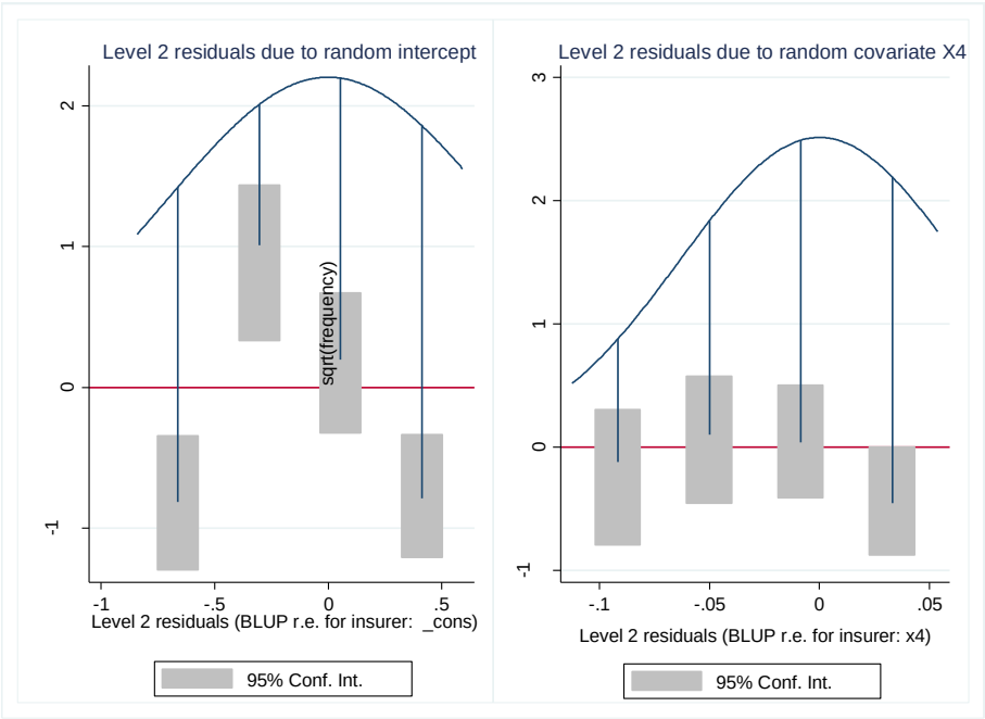
Figure 5: Rootograms for level-2 residuals
