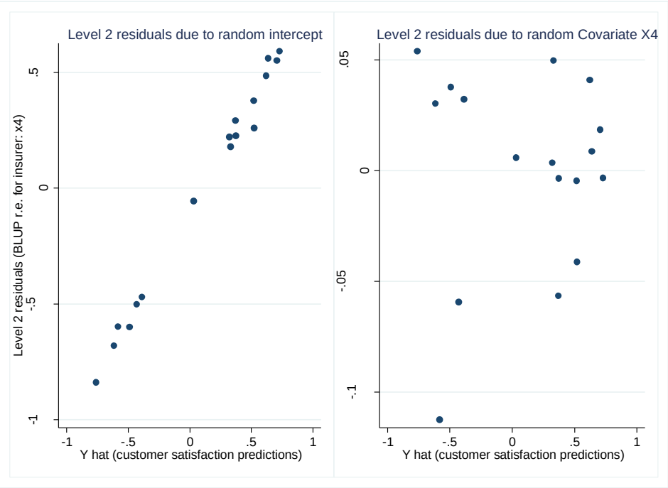
Figure 7: Scatter plot of residuals against predicted values for level-2 residuals
