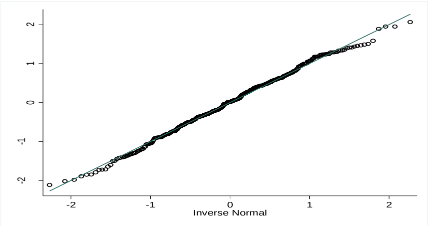
Figure 2: Q-Q plot for level-1 residuals
