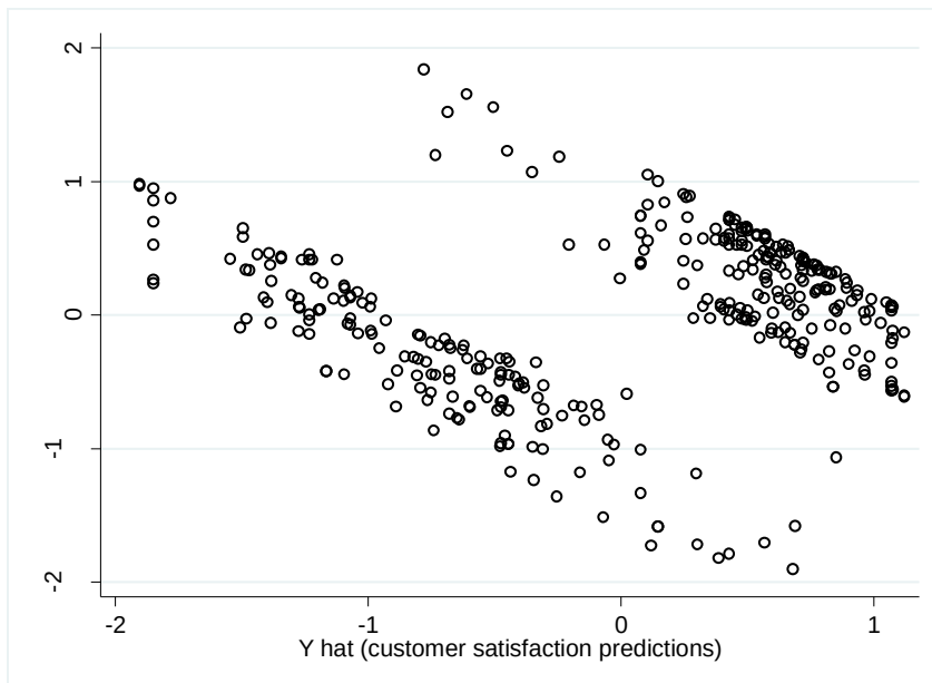
Figure 6: Scatter plot of residuals against predicted values for level-1 residuals
