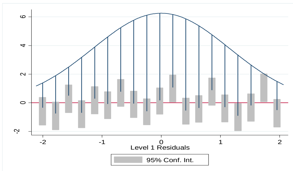
Figure 3: Rootogram for level-1 residuals; Service Blue Print against Customer Satisfaction Model
