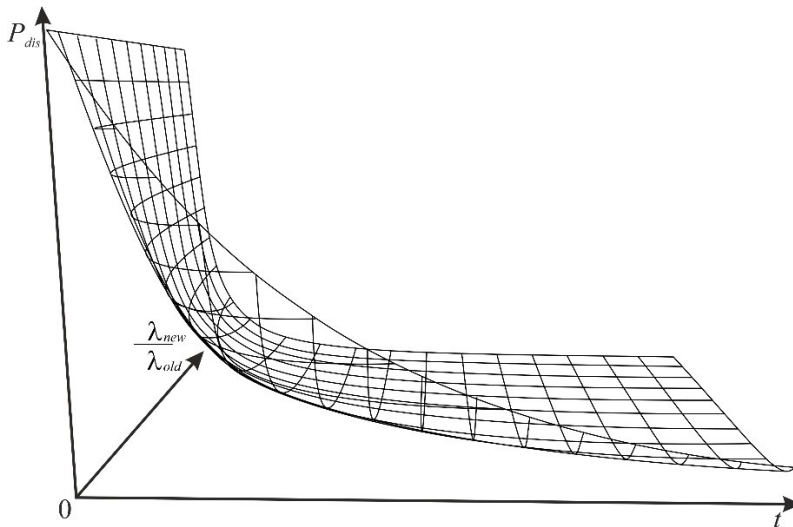
Fig. 3. Dynamics of changing probability of data entry into ITS element of another SSW version with divergences of information flows of different ITS versions: P_{dis} means probability that data arrive at ITS element from another
