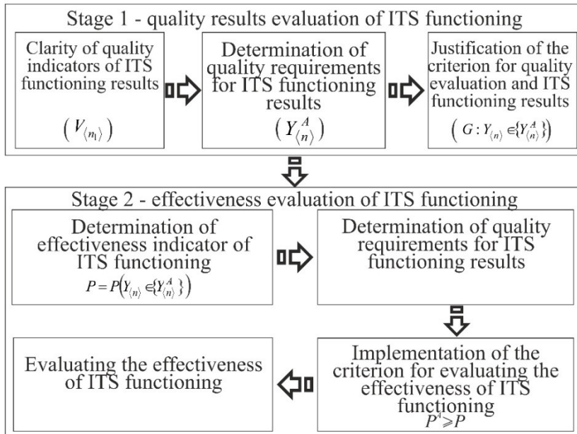
Fig. 1. Steps of evaluating the effectiveness of ITS functioning
