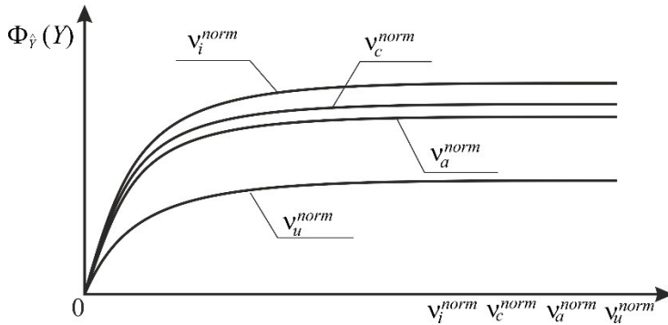
Fig. 4. Dynamic changes of probability values of performing functional tasks at partial changes of normative values: \Phi_Y(Y) is an effectiveness of performing ITS functional tasks, v_i^{norm} - normative value of the integrity indicator, v_c^{norm} - normative value of the confidentiality indicator, v_a^{norm} - normative value of the accessibility indicator, v_u^{norm} - normative value of the observation indicator
