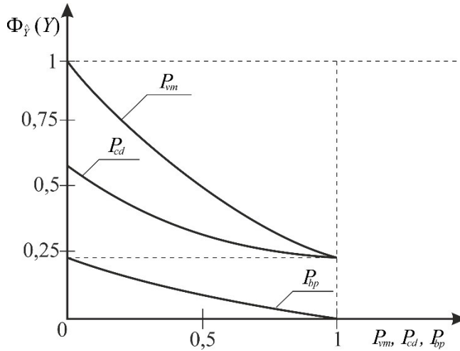
Fig. 6. Dynamic change of values of probability of performing functional tasks by the information system at separate components change: \Phi_{\hat{Y}}(Y) is an effectiveness of completing ITS functional tasks, P_{vm} - probability of SSW versions mismatch, P_{cd} - probability of a certain category data delivery in ITS, P_{bp} - probability that certain category data come into the general field of an ITS element from the old or new SSW versions with broken properties
