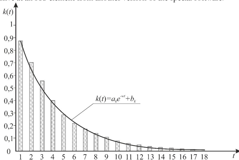
Fig. 2. Dynamics of changing probability of data entry into ITS element from other version of special software: k(t) is an upgrading part, t - upgrading time, w, a_k, b_k are parameters of realization speed of upgrading ITS components
